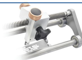
Robust bronze knobs for "fast traverse" & blade positioning
